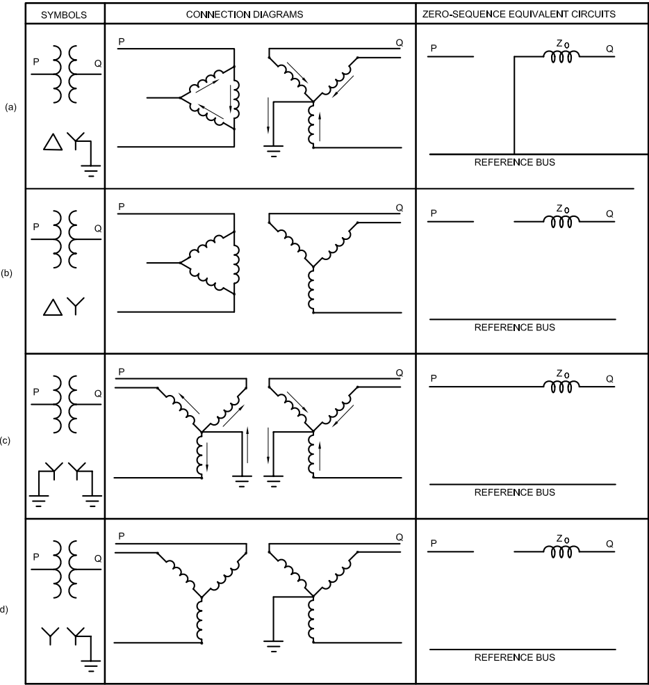
Figure 1-18—Zero-sequence impedance of different transformer configurations
