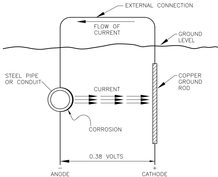
Figure 4-2—Galvanic cell—dissimilar metals
