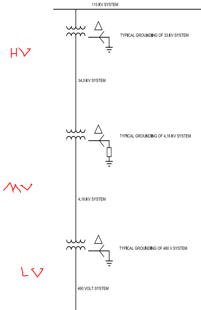
Figure 1-4—Independent grounding of each voltage level
